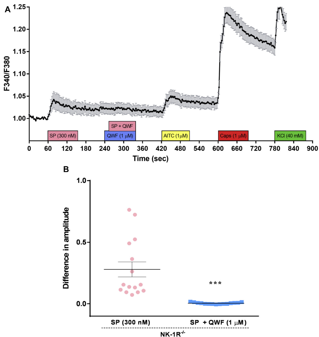
FIG 4. Effect of QWF on SP-induced \text{Ca}^{2+} flux in cultured DRG neurons from \text{NK-1R}^{-/-} mice. A , QWF (1 \mu\text{mol/L} ) blocks SP-induced (300 \text{nmol/L} ) \text{Ca}^{2+} flux in DRG neurons from \text{NK-1R}^{-/-} mice. Cells blocked by QWF also respond to allyl isothiocyanate (1 \mu\text{mol/L} ), capsaicin (1 \mu\text{mol/L} ), and KCl (40 \text{mmol/L} ). B , Amplitude of SP-induced \text{Ca}^{2+} flux in \text{NK-1R}^{-/-} neurons before and after treatment with QWF (1 \mu\text{mol/L} ). Data are expressed as means \pm SEMs. The paired Student t test was used. Statistical difference from SP is indicated as follows: *** P < .001 . Total number of cells analyzed was as follows: Fig 4, A, 314; Fig 4, B, 492.
