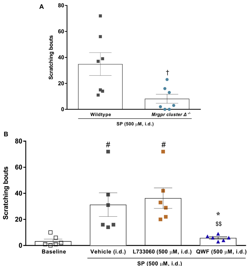
FIG 1. Mrgprs mediate SP-induced itch. A , SP-induced itch (500 \mu\text{mol/L} administered intradermally [ i.d. ]) is significantly decreased in Mrgpr cluster Δ -/- mice. B , Effects of treatment with the NK-1R antagonist L733060 (500 \mu\text{mol/L} administered intradermally) or the dual NK-1R/Mrgpr antagonist QWF (500 \mu\text{mol/L} administered intradermally) on scratching behavior caused by SP (500 \mu\text{mol/L} administered intradermally). Data are expressed as means \pm SEMs. The unpaired Student t test ( n = 7 mice per group in Fig 1, A ) and 1-way ANOVA followed by the Tukey test ( n = 6 mice per group in Fig 1, B ) were used. Significant differences from wild-type mice ( \dagger P < .05 ), baseline ( \#P < .05 ), SP plus vehicle ( *P < .05 ), or SP plus L733060 ( \$P < .01 ) are indicated.
