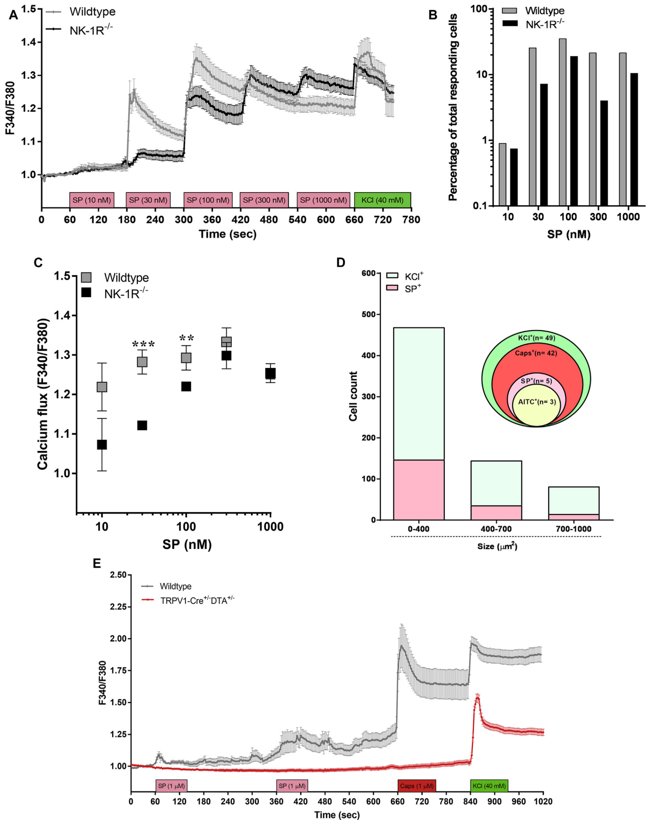
FIG 3. SP activates NK-1R -/- nociceptors. A , SP (10-1000 nmol/L) induces Ca 2+ flux in wild-type (gray) and NK-1R -/- (black) cultured DRG neurons. B , Percentage of SP-responding cells from wild-type or NK-1R -/- mice. C , Maximal Ca 2+ flux in DRG neurons from wild-type (gray) and NK-1R -/- (black) mice. D , Size of SP-responsive cells from NK-1R -/- mice. Inset , Venn diagram showing overlapping populations of KCl-positive, capsaicin-positive, and SP-responsive neurons. E , Ca 2+ flux induced by SP (1 μmol/L), capsaicin (1 μmol/L), and KCl (40 mmol/L) in DRG neurons from wild-type (gray) and TRPV1-Cre +/+ DTA +/- (red) mice. The unpaired Student t test was used. Significant differences from NK-1R -/- were indicated as follows: ** P < .01 and *** P < .001. Total number of cells analyzed was as follows: Fig 3, A-C, 328 (wild-type) and 1463 ( NK-1R -/- ); Fig 3, D, 1463; Fig 3, D, inset , 314; and Fig 3, E, 787 (wild-type) and 246 (TRPV1-Cre +/+ DTA +/- ).
