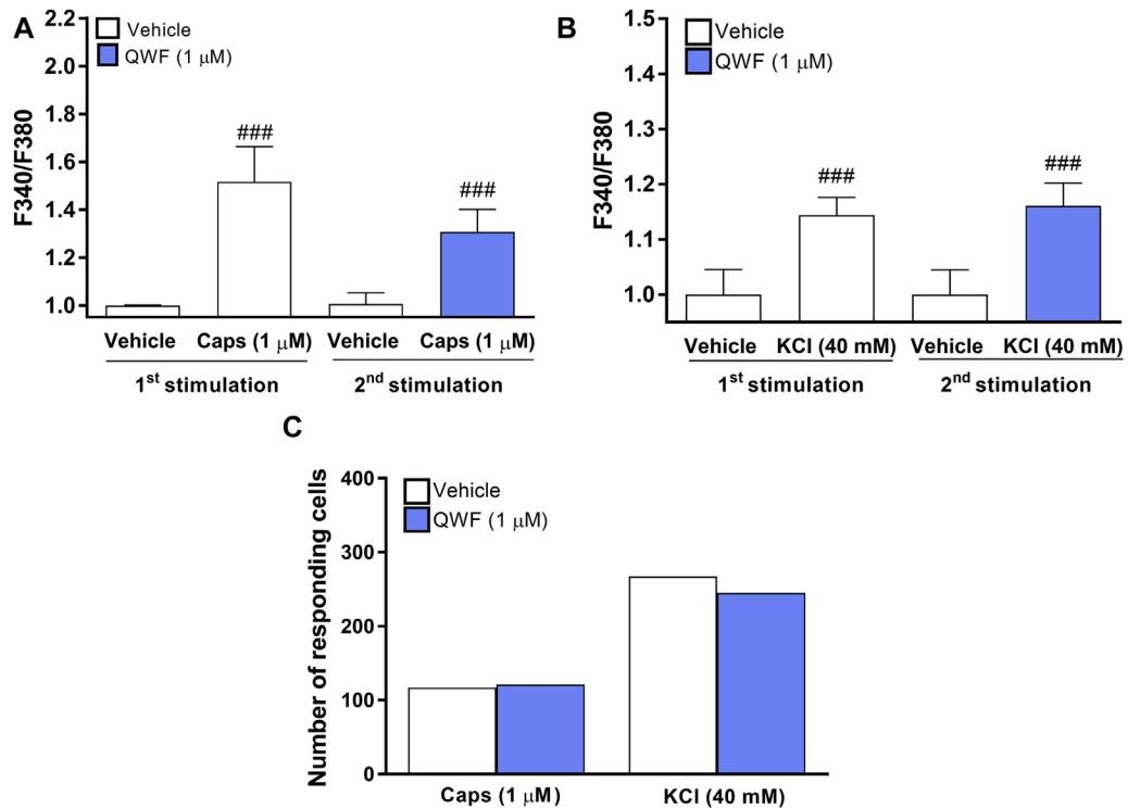
FIG E1. QWF does not affect capsaicin- or KCl-induced calcium flux. \text{Ca}^{2+} amplitude ( A and B ) and number of responsive cells ( C ) to capsaicin (Fig E1, A and C ; 1 \mu\text{mol/L} ) or KCl (Fig E1, B and C ; 40 \text{mmol/L} ) after treatment with QWF (1 \mu\text{mol/L} ) or vehicle are shown. Data are expressed as means \pm SEMs. The paired Student t test was used. Significant differences from vehicle are indicated as follows: ###P < .001 . Total number of cells analyzed was 267.
