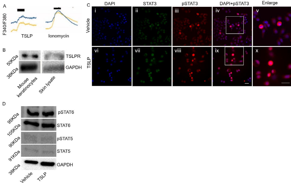
Figure S4. Expression of TSLPR/IL7R \alpha receptor complex and translocation and detection of STAT phosphorylation by Western blotting, related to Figure 7. A) Representative traces of calcium influx of TSLP (2ng/ml) and ionomycin (10 \mu M) on mouse keratinocyte cell line that were cultured for 24 hrs, n=3 coverslips from independent preparation. B) Skin immunoblot showed the expression of TSLPR in mouse keratinocytes cell line and skin. Data were repeated three time with similar results. C) TSLP-mediates the translocation of pSTAT3 in mouse keratinocytes. There was no change in the expression of totalSTAT3 (ii and vii), whereas the activated form, pSTAT3, transported to the nucleus in response to 10ng/ml TSLP (ix compared to iv [PBS control]). Outlined images iv and ix are further magnified (v and x). Data were repeated three time with similar results. Scale bar 25 \mu m. D) Representative immunoblot of both phosphorylated and non-phosphorylated STAT5 and STAT6, which shows no change in in response to TSLP (10ng/ml) compared to vehicle (PBS) treated. Samples were probed with antibodies against pSTAT5, pSTAT6, STAT5, STAT6, and GAPDH, n=3 mice.
