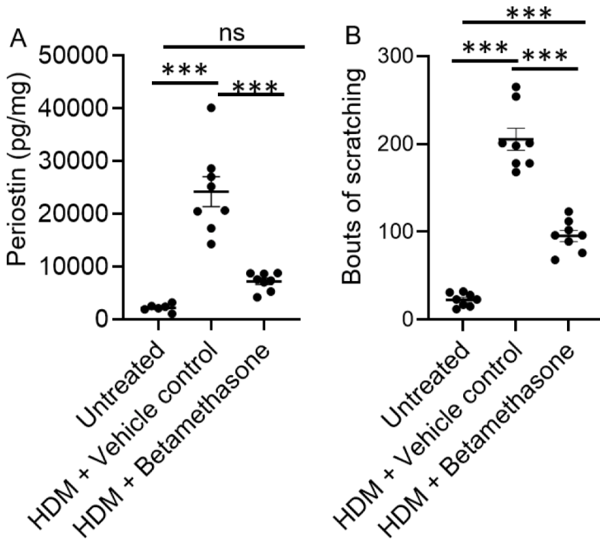
Figure S5. HDM-induced periostin in the skin and itch in AD mouse model, related to Figure 7. A) NC/Nga mice were topically applied with Dermatophagoides farinae HDM (10mg/ml) and ELISA was performed on the skin tissue homogenates to measure periostin and compared that to mineral oil. A significant decrease in periostin production in mice treated with glucocorticoids betamethasone compared to vehicle treated group, n=8 mice. B) A significant increase in scratching bouts observed in NC/Nga mice applied topically with allergen HDM (10mg/ml) compared to mineral oil. The scratching behavior was significantly reduced in mice treated with glucocorticoids betamethasone compared to vehicle treated group, n=8 mice. All data were represented in mean \pm SEM, Significant difference between more than two groups were performed using one-way ANOVA with Dunn's test (***) p <0.001).
