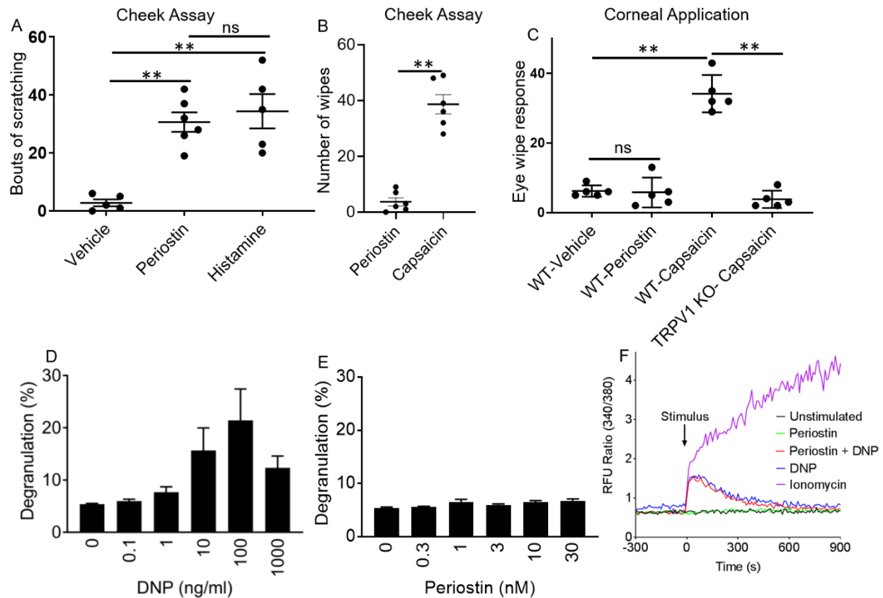
Figure S1. Periostin evoked itch behavior but not pain directly through sensory neurons, related to Figure 1.
