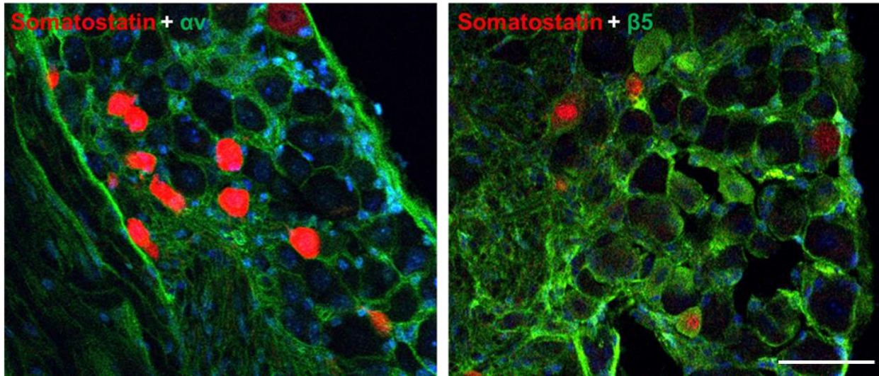
Figure S2. Integrin receptor subunit \alpha v and \beta 5 expression in the dorsal root ganglia, related to Figure 2. Double IHC illustrates the expression of the integrin receptor \alpha v and \beta 5 subunit (green) in majority of sensory neurons and SST-positive neurons are small subset (red). Data were repeated three time with similar results. Scale bar 75 \mu m.
