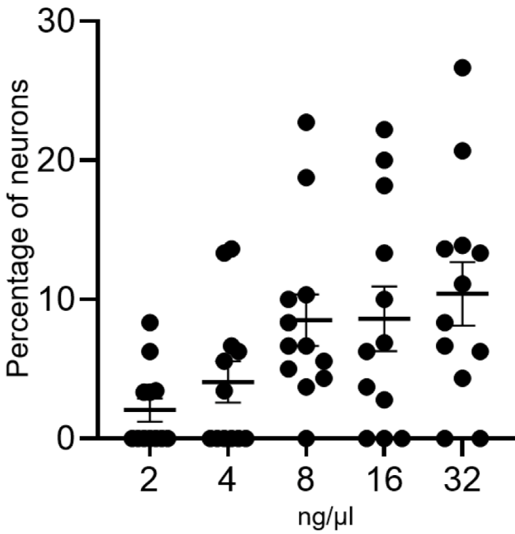
Figure S3. Concentration-dependent calcium influx to periostin, related to Figure 3. Periostin-evoked calcium response is concentration dependent. A dot point in calcium imaging scatter plot represents one coverslip. All data were presented as mean \pm SEM, n=3 mice.
